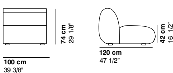
COD.1468 ELEMENT 100
