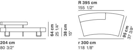
COD. 8462SXN CLOSED ELEMENT LEFT HALF BACK R 395
