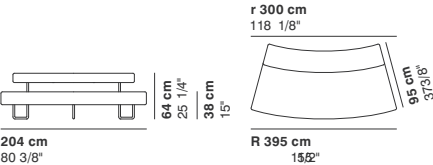
COD. 8461N OPEN ELEMENT CURVED R 395
