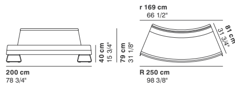
COD. 4014N OPEN ELEMENT CURVED 200
