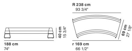
COD. 4019N CLOSED OTTOMAN CURVED 188
