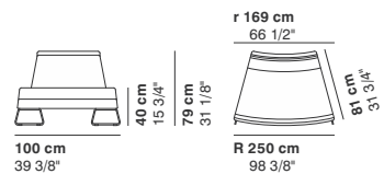
cod. 4012 / open element curved 100
