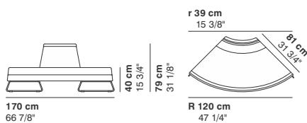
cod. 4017 / open element curved 90°
