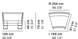
cod. 4013 / closed element curved 100
