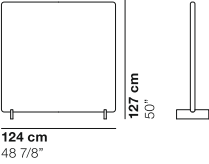
COD.1344 UPHOLSTERED LOW SCREEN
