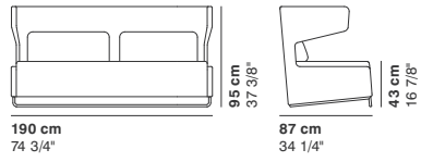
COD. 8107N 2 SEATER SOFA MAJOR
