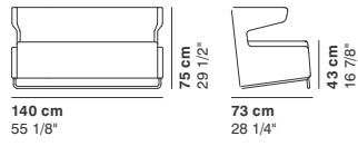
COD. 8107N 2 SEATER SOFA MAJOR
