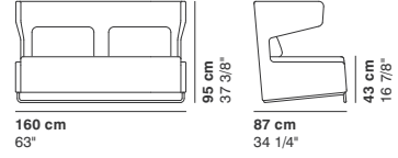
COD. 8108N 3 SEATER SOFA
