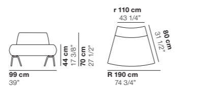
cod. 1187 / open element 30° R190
