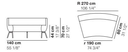
cod. 1190 / closed element 30° R270
