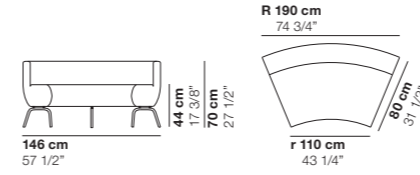
cod. 1188 / closed element 45° R190
