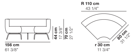
cod. 1182 / closed element 90° R110
