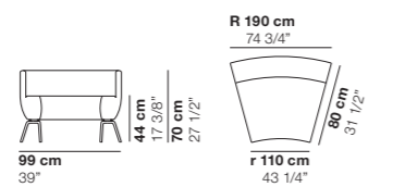
cod. 1186 / closed element 30° R190
