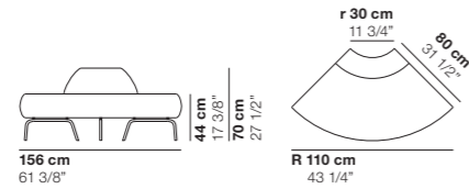
cod. 1183 / open element 90° R110
