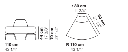
cod. 1185 / open element 60° R110
