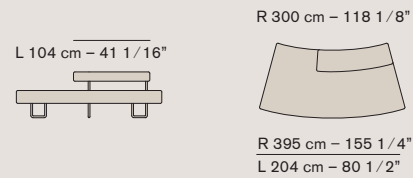
element open curved R395 - half back DX / cod. 8464DX
