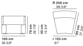
cod. 9016 / closed element curved 100
