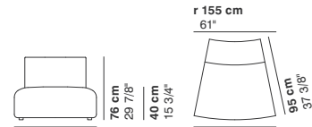
cod. 9015 / open element curved 100
