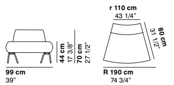
COD.1187 OPEN ELEMENT 30° R190
