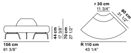
COD.1183 OPEN ELEMENT 90° R110
