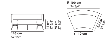
COD.1188 CLOSED ELEMENT 45° R190
