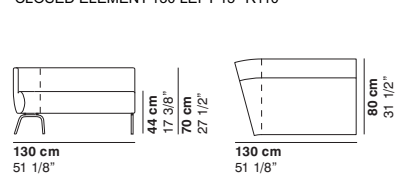
COD.1194 CLOSED ELEMENT 130 LEFT 15° R110
