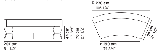
COD.1192 CLOSED ELEMENT 45° R270
