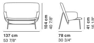
COD. 8905 WOOD_LOW ARMCHAIR CAPITONNE'
