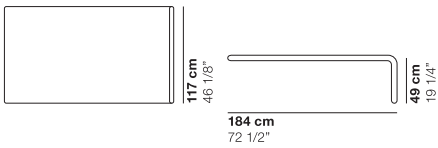
cod. 1334 / acoustic back round corner
