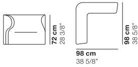
cod. 1317 / free upholstered back
